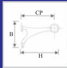
#104 Plain Floor Mount Bracket
