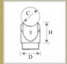
#726 35° H.Connector
