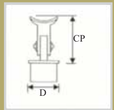
#711 Adjustable Saddle
